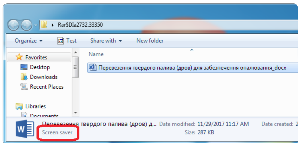
Figure 3 // Executable file disguised as a Word document.
